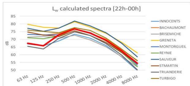
Figure 5 : Acoustic power level spectra ( L_w/m^2 ) determined to characterize the recreational activity surrounding each measurement point for the time slot [10 p.m.-12 a.m.]. In red, the average spectrum chosen for application in the model.
