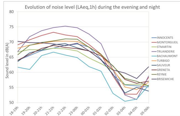
Figure 4 : Evolution of noise level ( L_{Aeq,1h} ) during the evening and night.
